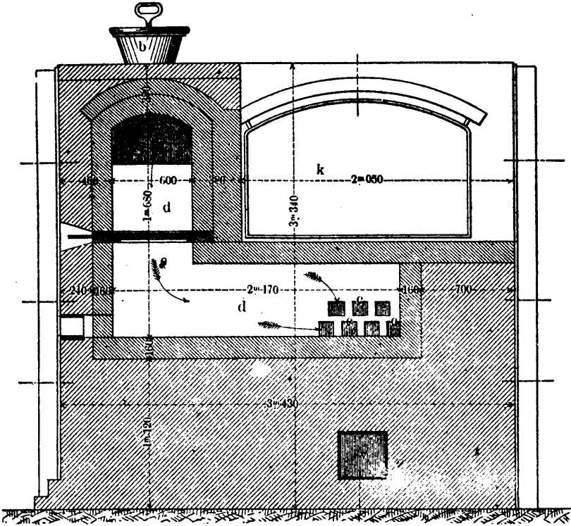
Fig. 1.—Vertical Cross Section near End.—Shown by C D in Fig. 4.
