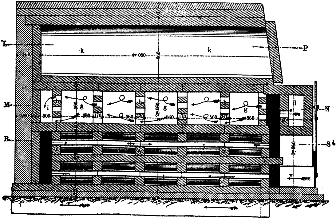
Fig. 2.—Longitudinal Section through Muffle.—Shown by A B, Fig. 4.
