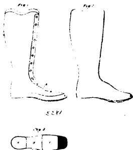
2281 Briggs's Improvement in Gaiters.
