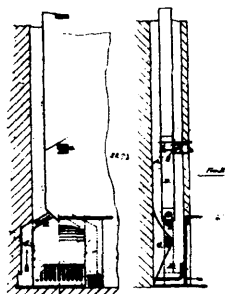
2293 Gray's Fire-Place Heater.
