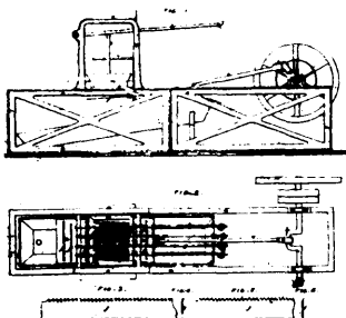
2290 Nood's Manufacture of Paper Pulp.
