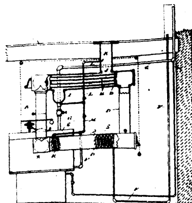
34135 King's Steam Heating Apparatus.
