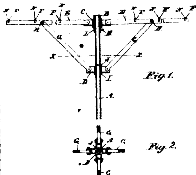
34127 Richmond's Clothes Drying Reel.
