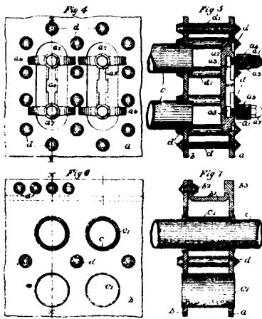
31960 Taylor's Steam Boiler.
