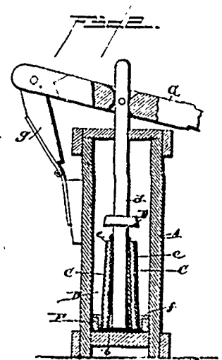
29403 Benjamin's Churn.
