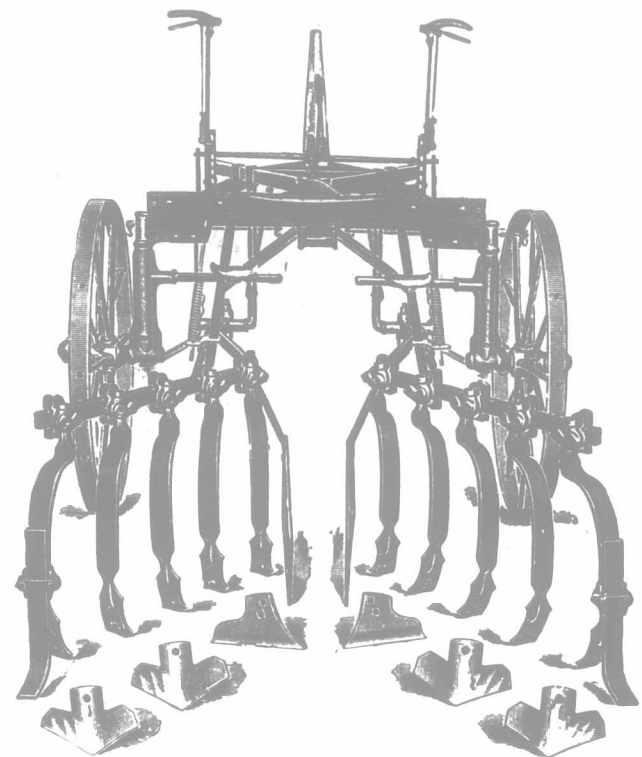
Above is shown Frost & Wood Climax Cultivator. Below is the Cockshutt Western Spring Tooth, adapted for either Field or Row Crop Cultivation—two machines in one.
