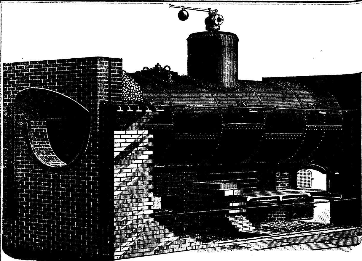
THE BIGELOW RETURN-TUBE BOILER.
