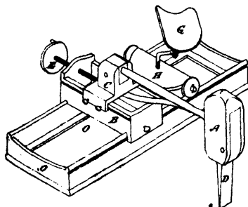
7436 Young's Machine for Dressing Mill Stones.
