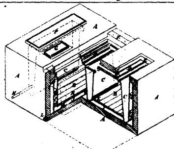
7430 Armstrong's Improvements in Preserving Chambers.
