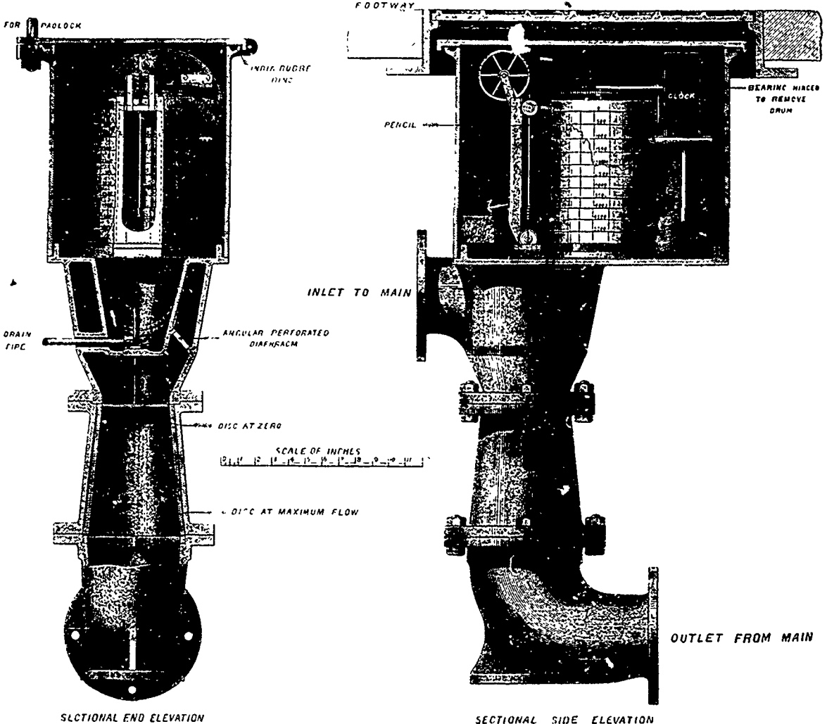
WASTE WATER METER. (See page 282.)
