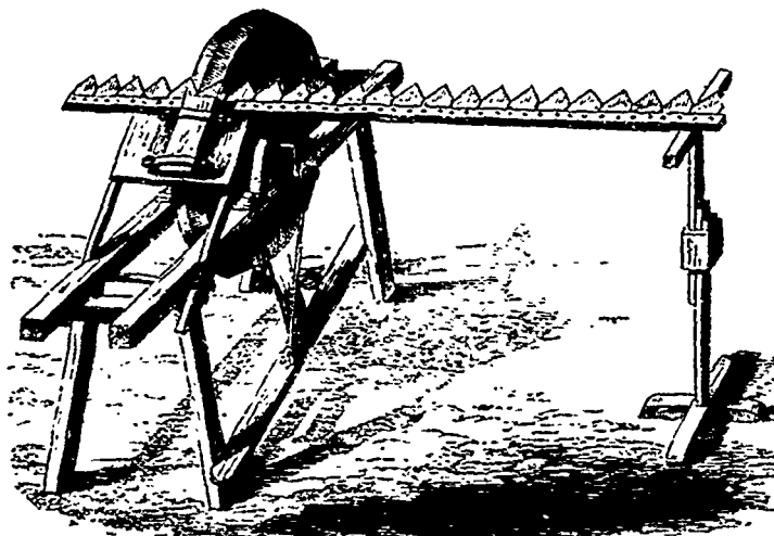
Fig. 3.--GRINDING MOWER-KNIFE.
