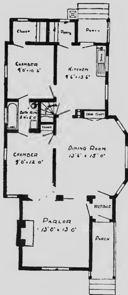
FLOOR PLAN
