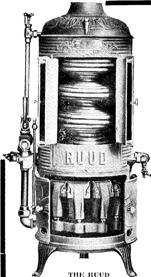
THE RUUD Showing Heating Coils and Burners.
