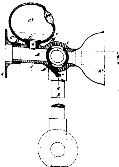
Cutmore's Speaking Tube.
