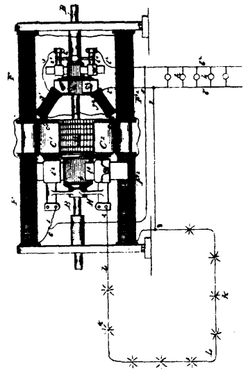
27037 Easton's Dynamo Electric Machine.
