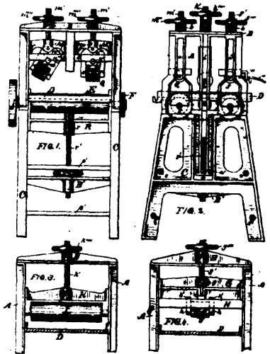
27041 Burdett's Machine for Ornamenting Wood, etc.
