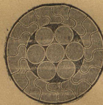
Locked Coil Aerial Cable or Colliery Guide.
