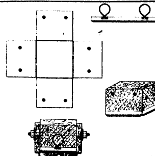
4782 Hagan, Bryce, & Gibson's Manufacture of Concrete Blocks Veneered with Marble.
