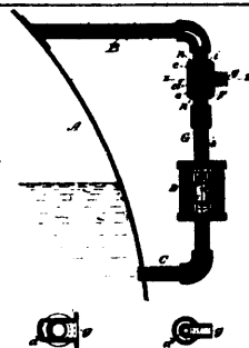
4779 Henry's Regulators for Feed Apparatus.
