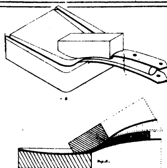
4776 Blake's Mode of Manufacturing Shovels.
