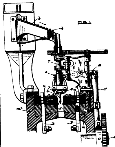
32614 Rogers' Mode of Forming Screw Threads.
