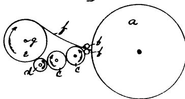
32610 Connelly's Machine for Carding Cotton.
