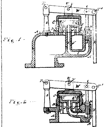
26770 Pendy's Balance Throttle Valve.
