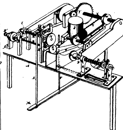
18576 West's Apparatus for Crimping the ends upon Circular Cans and preparing them for Soldering.
