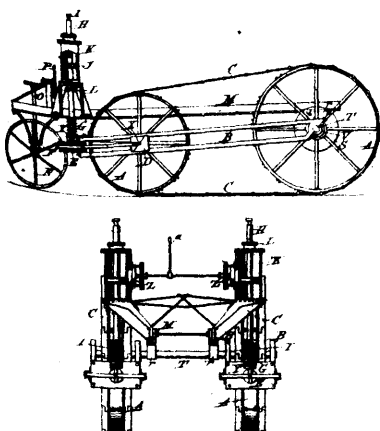
Hanscom's Traction Attachment for Road Engines.
