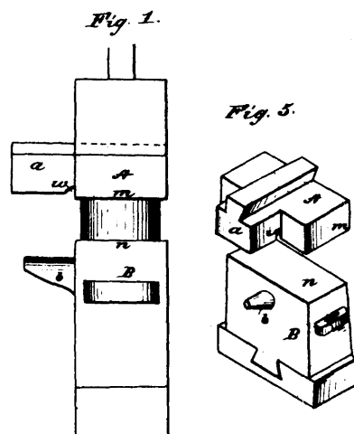
18679 Facer & Schaub's Device for Manufacturing Car Wheel Tires.
