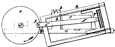
14177 Smith's Improvements in Veneer Cutting Machines.
