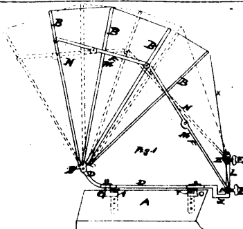
14185 Hodge's Improvements on Carriage Tops.
