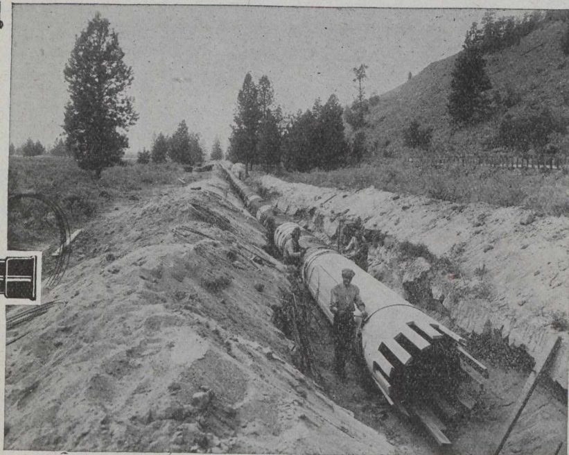
48 in. CONTINUOUS STAVE LINE.
