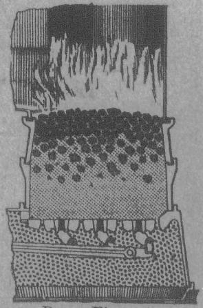
Pease Fire-pot.
