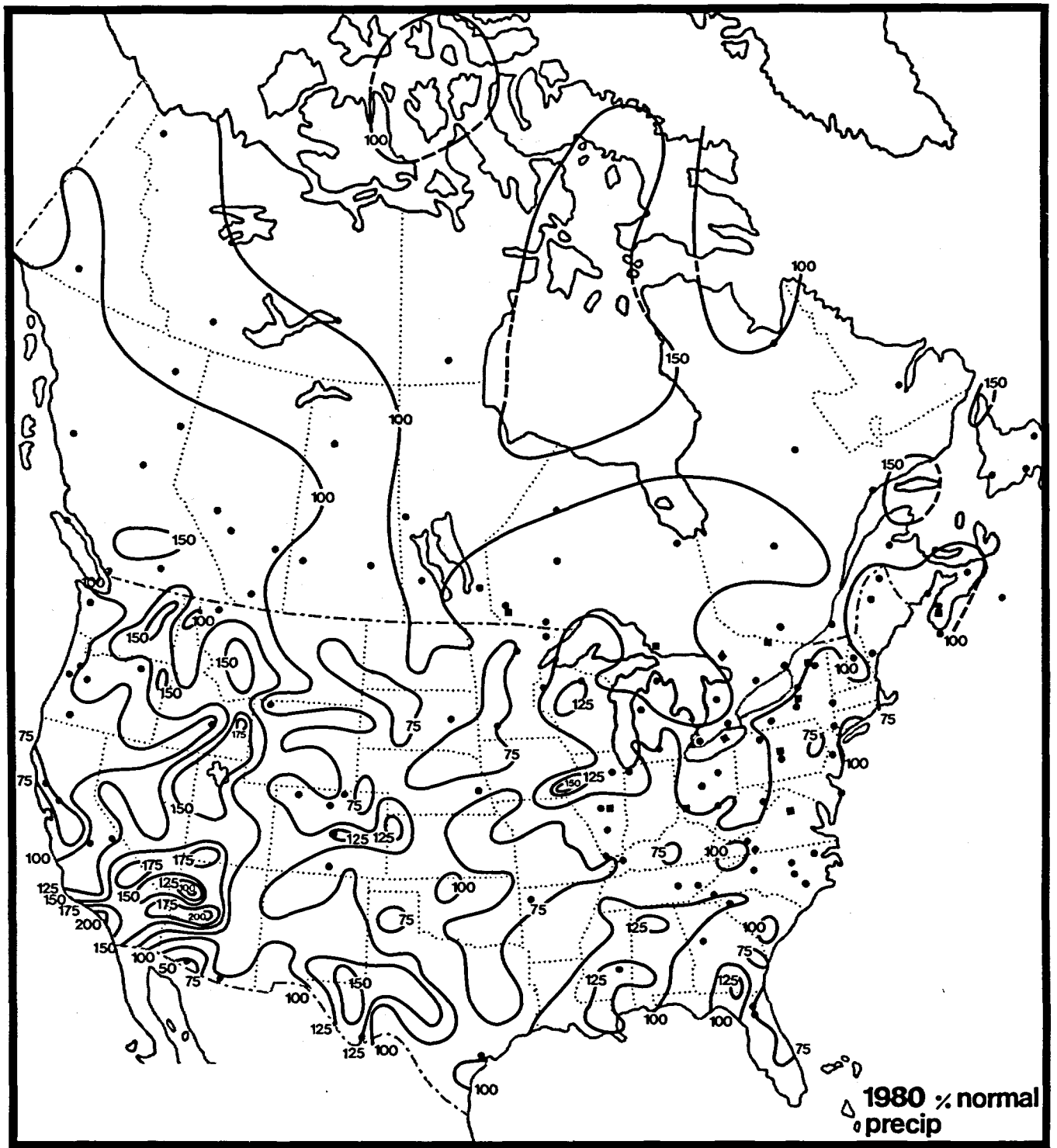
Percent of normal precipitation in North America in 1980
