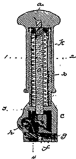
23010 Walter &amp; Bender's Stamp Canceller.
