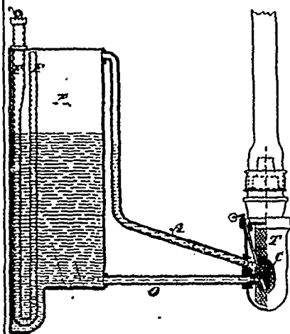
23011 Livesey's Oil Lamp.
