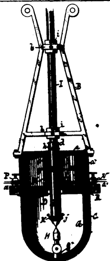
18608 Edgerton's Electric Arc Lamp.
