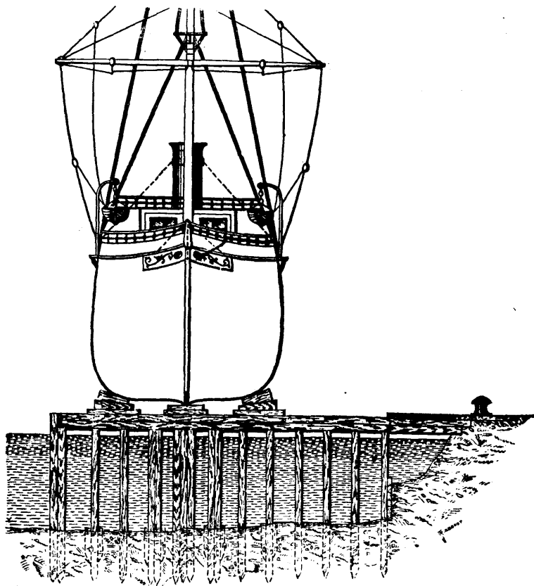
FIG. 3. VESSEL DEPOSITED ON STAGING.
