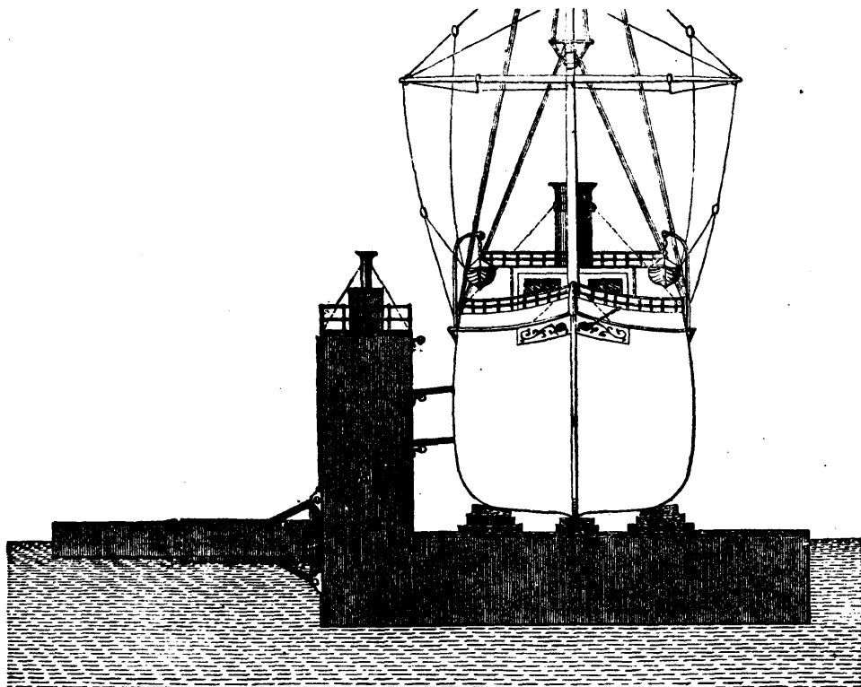
FIG. 2. DOCK-FLOATING, WITH VESSEL RAISED.
