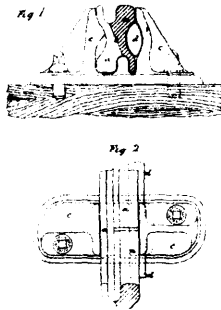
9211 Aldred's Improvements in Railway Rails.
