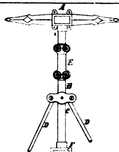
8557 Morrison's Improvements in the Gear of Buggies.
