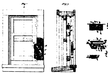
8554 Rush's Improvements on Sash Fasteners.
