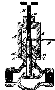
3491 Allmand's Valve-Seat Refitting Machine.
