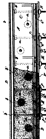
41756 Pruyn's Electric Railway.
