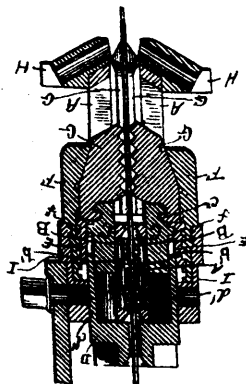
Robinson and Watt's Machine for uniting Soles and Uppers of Boots.
