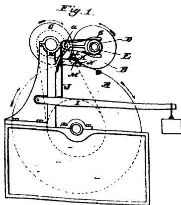
Fairbanks and Parker's Machine for forming Bodies from Successive layers of Pulp.
