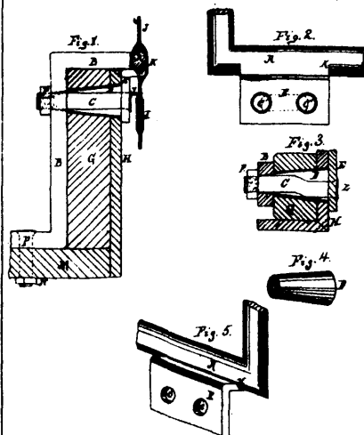
15709 Elliott and Lance's Improvements in Vehicle Dashes.
