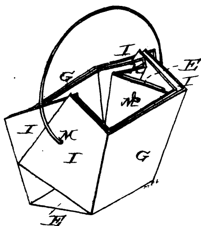
15707 Smith's Improvements on Boxes for Berries.
