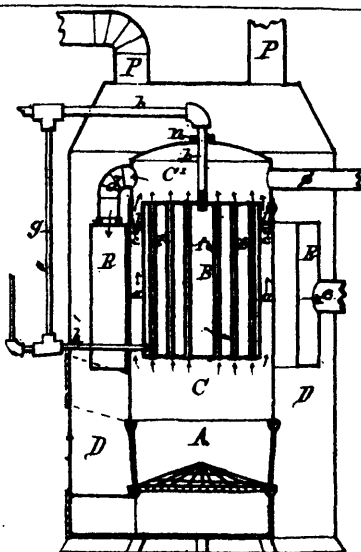
15708 Pease's Improvements on Heating Apparatus.
