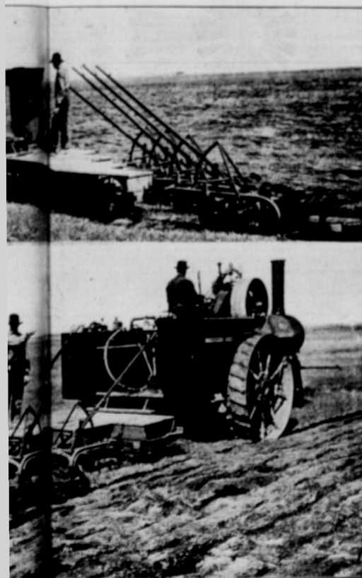
Simple Mount Tricycle Type Special Plowing Engines in action gumbo at the Walker Farm, near Warren, Manitoba.
