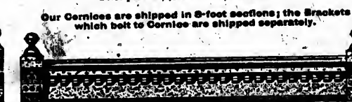
No. 671. Height, 36 inches; Proj., 12 inches. Price per foot, 70c. Urns, 60c each.
