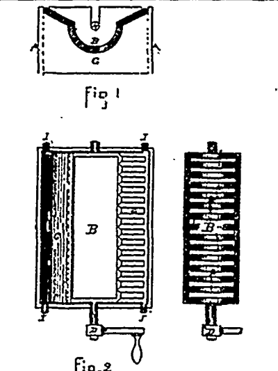
23511 Copp's Fire Place Grate.
