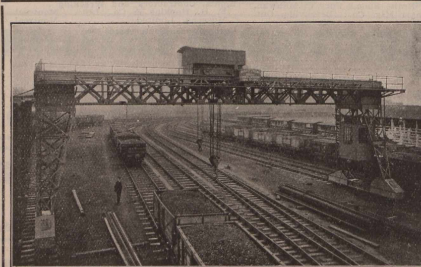
The G. & S. W. Rwy., Albert Harbor Goods Station, Greenock, N.B. "B. & W." 30 Tons Electric Travelling Goliath Crane, 70 Feet Span
