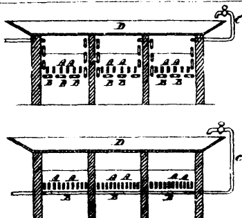
Hayes's Tubular Brine Evaporator.
