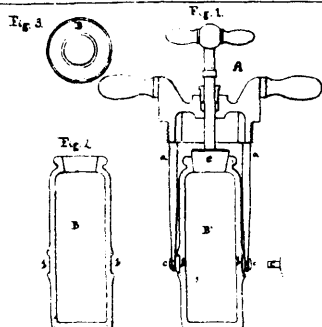
Kley's Chemical Fire Extinguisher.
