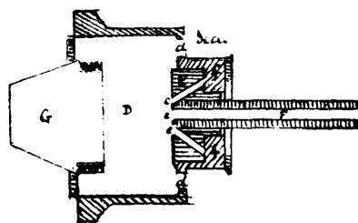
2390 Parson, Barret &amp; Marwick's Petroleum Burner.
