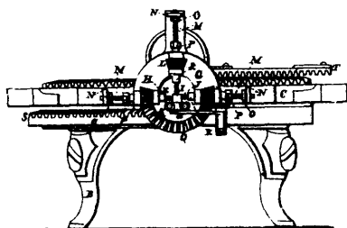
Pope's Machine for Tapping Gas Fittings.
