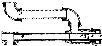
Whyte's Tar Burner.
