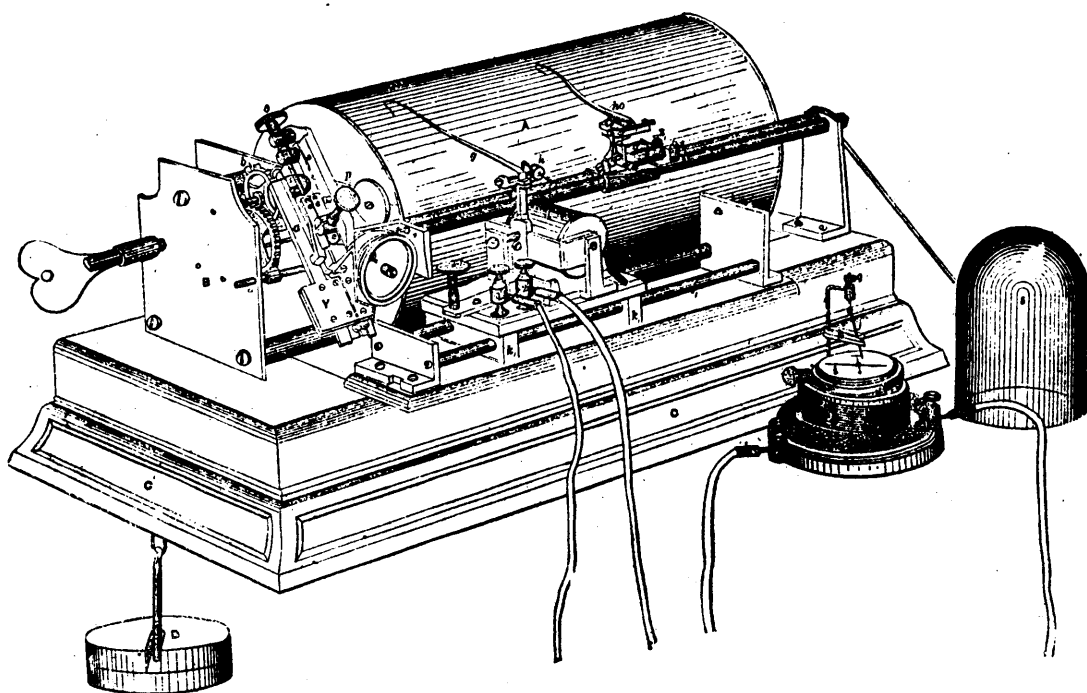
FIG. 1.—CHRONOGRAPH FOR ENGINEERING PURPOSES.
