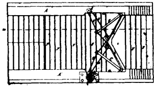
11565 Millette's Improvements in Lock Gates.
