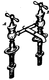
10811 Campbell's Improvements on Compression Cocks.
