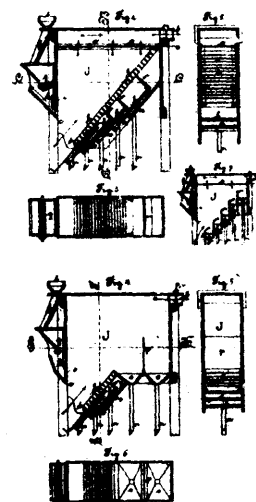
37848 Haggemacher's Apparatus for Purifying and Sorting Grits.
