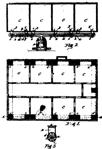
37846 Howard's Heating Apparatus.
