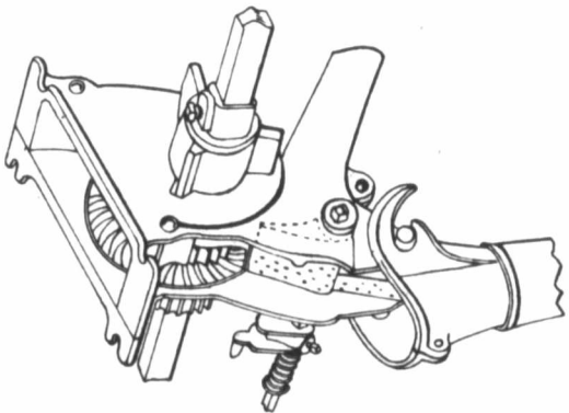
Fig. 1. Hoe Drill. Detail of Feed from Seed-box into the Tubes.
