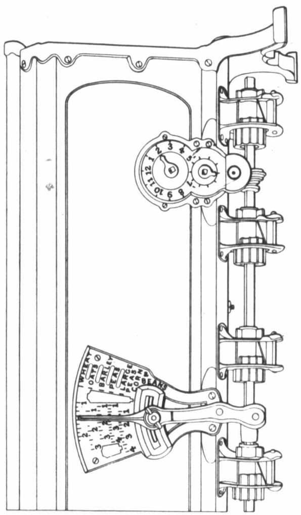
Fig. 2. Arrangement for Regulating the Flow of Seed, and Dial for Indicating Number of Acres Sown.
