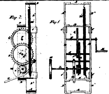
7811 Terrell's Improvements on Saw Grinders.
