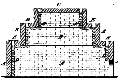
7810 Evans' Improvements on Brick Kilns.
