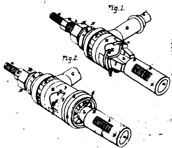
7807 Minshall's Improvements on Tube Expanders.
