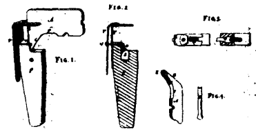
7808 Spaulding's Improvements in Saw Teeth.
