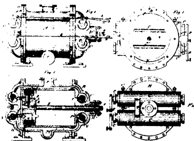
12347 Goodwin's Improvements on Steam Engines.
