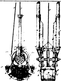
12352 Hall's Improvements in Dredging Scoops.
