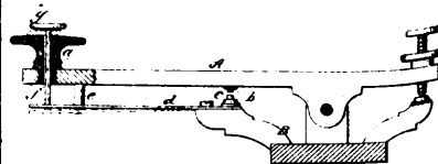
12358 Neilson's Improvements on Telegraph Keys-
