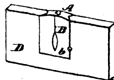
5309 Branch's Method of Inserting, Fitting and Securing Diamonds in Metallic Holders for Working in Stone.
