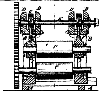
5306 Venner &amp; Rowley's Improvements on Machines for Rolling Tapered Bars.
