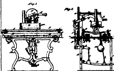
5296 Cottingham's Clothes Ironing Machine.
