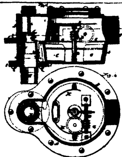
5308 Taylor &amp; Kimball's Water Meter.
