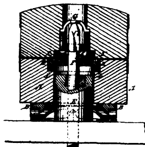
5302 Wallace's Improvements on Mill-tram.
