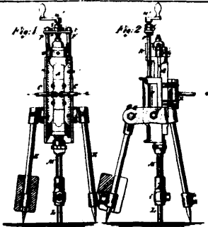
5061 Nutting &amp; Githens' Steam Drill.
