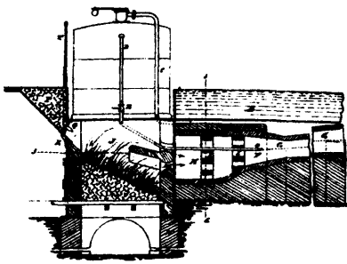
5058 Wilson &amp; Hayes' Evaporating Furnace.
