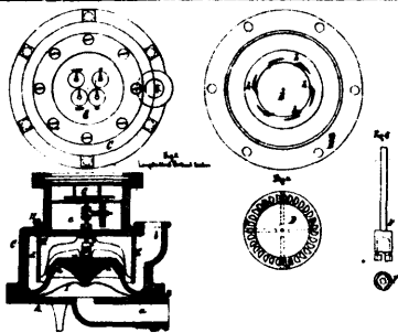
5067 Marsland's Liquid Meter.
