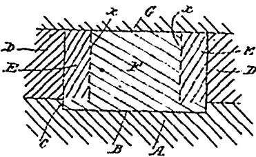
25630 Hatt's Brake Shoe.
