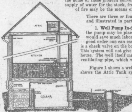
Figure 1—Hard and soft water system. Pump to well supplies hard water. Another pump sends soft water from cellar cistern to attic tank; this water can be piped all through the house.
