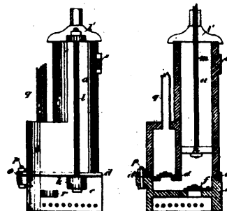
3616 Scott's Improvements on Force Pumps.
