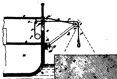
3613 Paterson's Portable Apparatus for Loading and Unloading Vessels.
