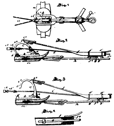
Howard's Check Rein Attachment.
